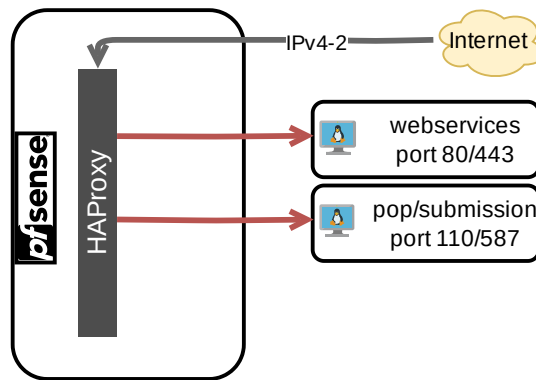
Webservices via HAProxy
